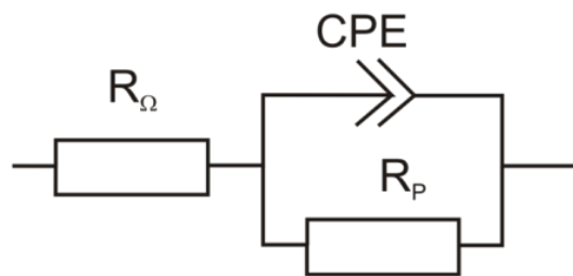
Fig. 6. Equivalent circuit for Bode plot with one minimum in Phase Bode plots.
